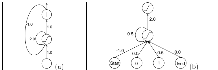
Fig. 2. (a) MSB encoder: A RNN that takes a real number between 0 and 1 and encodes it as a numeric string, most significant bit first. The hidden unit uses a linear threshold activation function that saturates at -1 and 1, whereas the output units use binary (0.5) threshold units. The input value is presented at the first time-step only. (b) LSB decoder: A SRN that decodes numeric sequences LSB first. The input is wrapped with start and end markers. After presentation of the end marker, the output unit activation corresponds to the appropriate value. Linear (0,1) threshold activations are used on all units.
